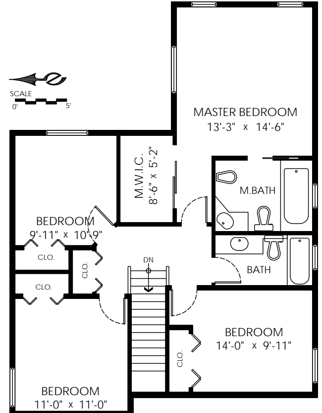
Upper Floor Plan Floor Area: 977 sq.ft.
